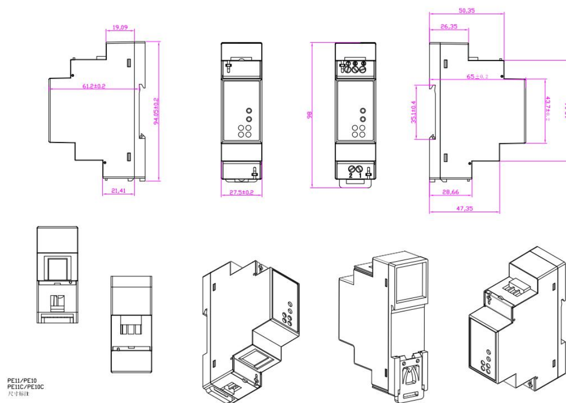
Figure 4. Protoss-PE11 Mechanical Dimension
