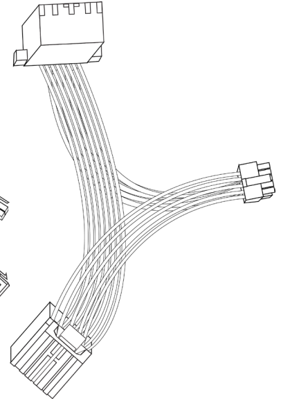
Vehicle Specific Plug and Play Harness (Part # NT-HA12)
